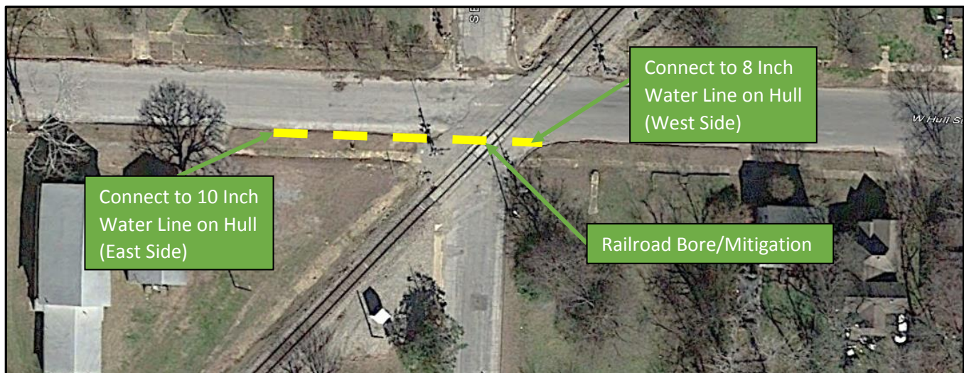
WEST HULL WATER LINE LOOP (Bore Under BNSF Railroad Tracks)
